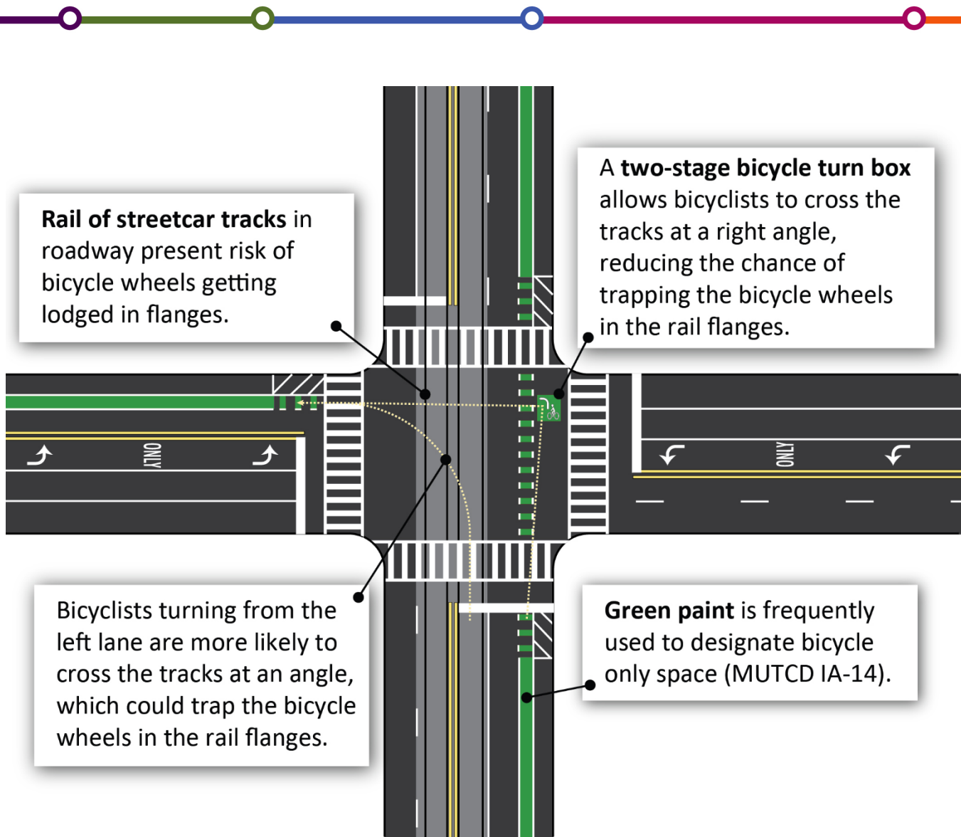
Figure 39. Graphic. Two-stage left turn for bicyclists crossing rail or streetcar tracks. (VHB, 2021).*
