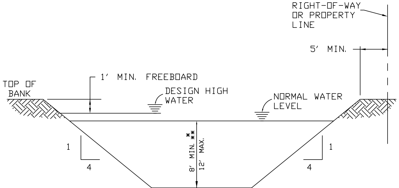
STANDARD DETENTION POND DETAIL PREFERRED OPTION
