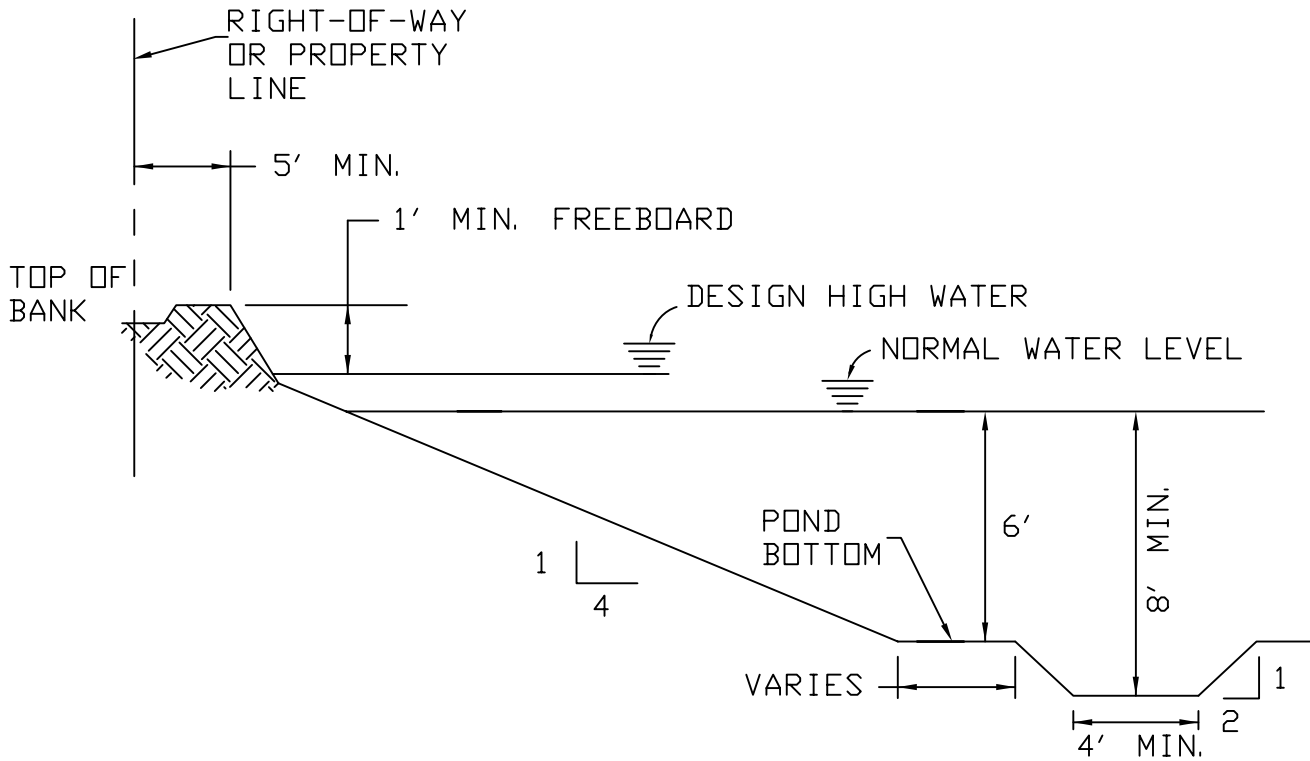
CASE 2 WET DETENTION POND DETAIL
