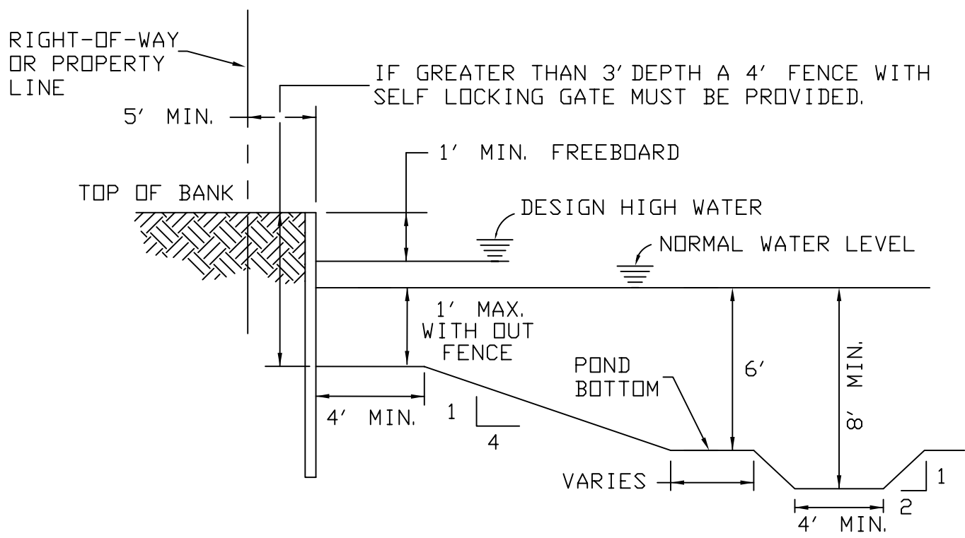
CASE 3 WET DETENTION POND DETAIL
