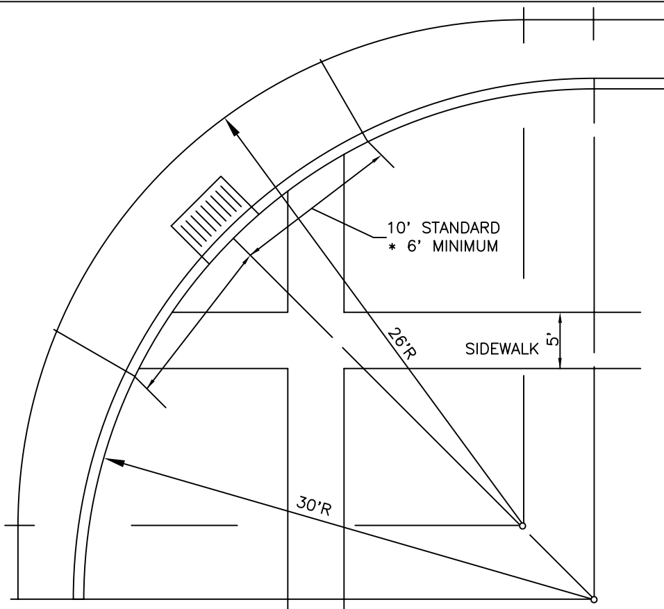
TYPICAL INSTALLATION ON CURB RETURN
