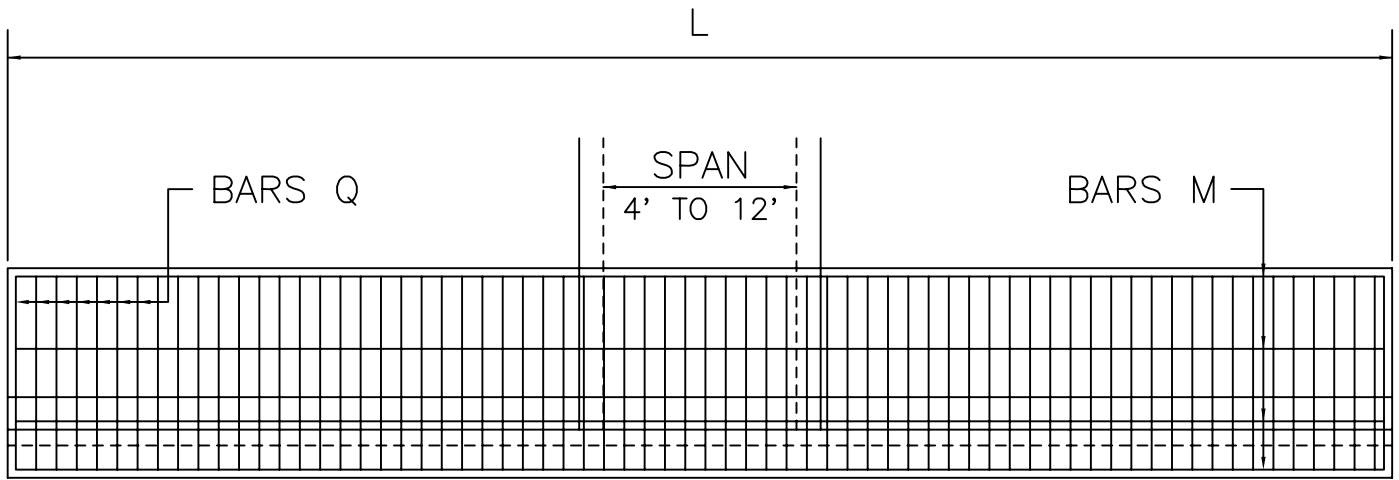
PLAN—SHOWING BARS IN FOOTING
