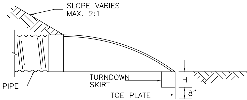
CROSS SECTION
