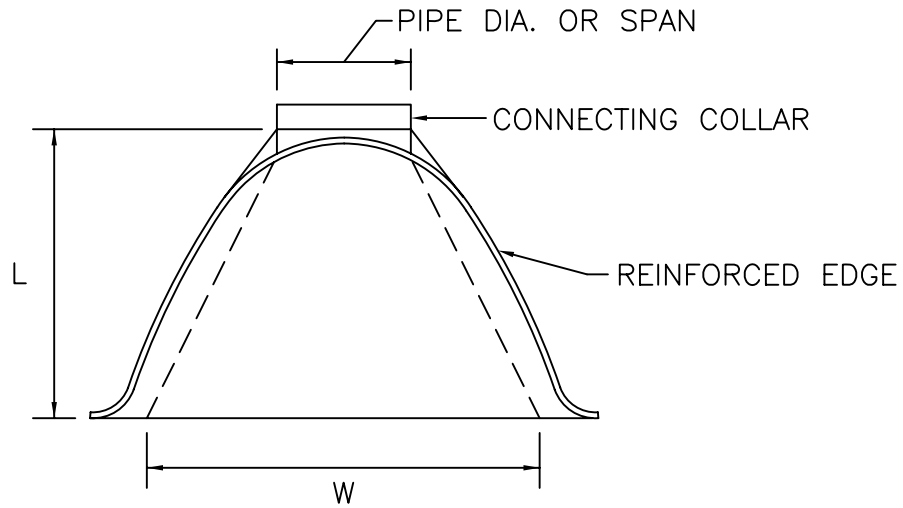
PLAN VIEW
