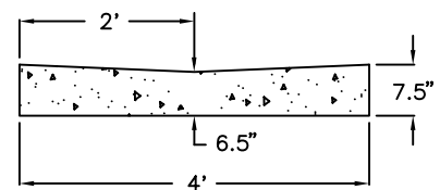
(Optional) TYPICAL CONC. VALLEY (MIN. 3500 PSI CONC.)
