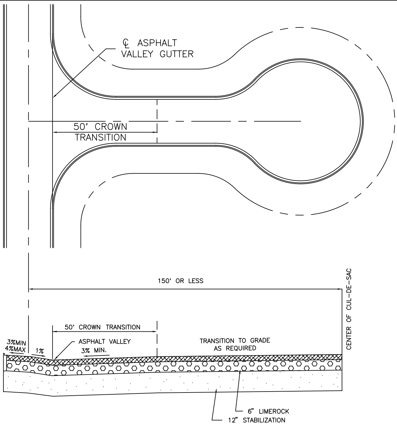
TYPICAL ASPHALT VALLEY GUTTER
