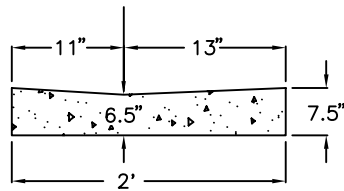
TYPICAL CONC. VALLEY (MIN. 3500 PSI CONC.)
