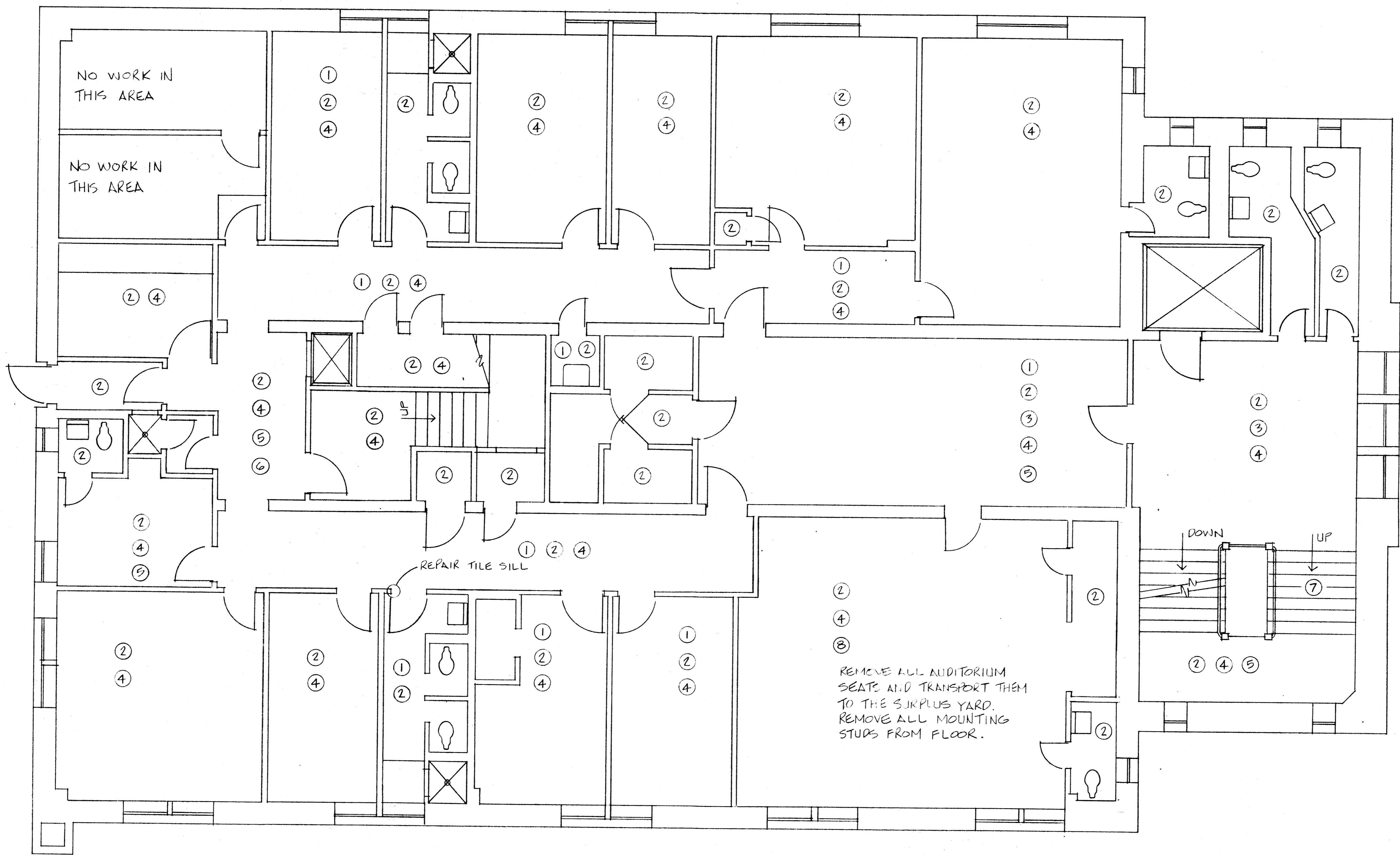
SECOND FLOOR PLAN \frac{1}{4}'' = 1'-0''
